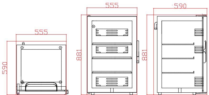
Recommended space required around cabinet (with remote mounted compressor) to allow for sufficient air circulation: 555(w) x 881(h) x 590d)mm
